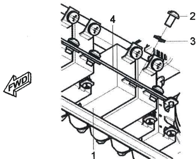
Figure 9 - Connection the new LDG L W31X2M1G-3 switch circuit breaker to the main supply bus.
